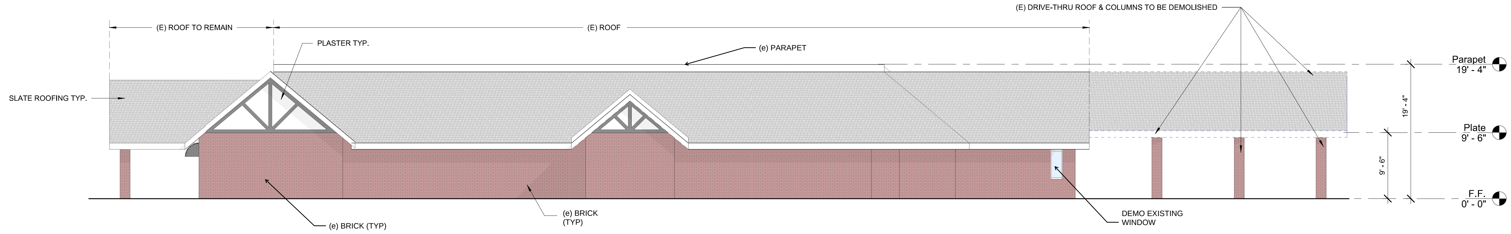
EXISTING WEST ELEVATION
