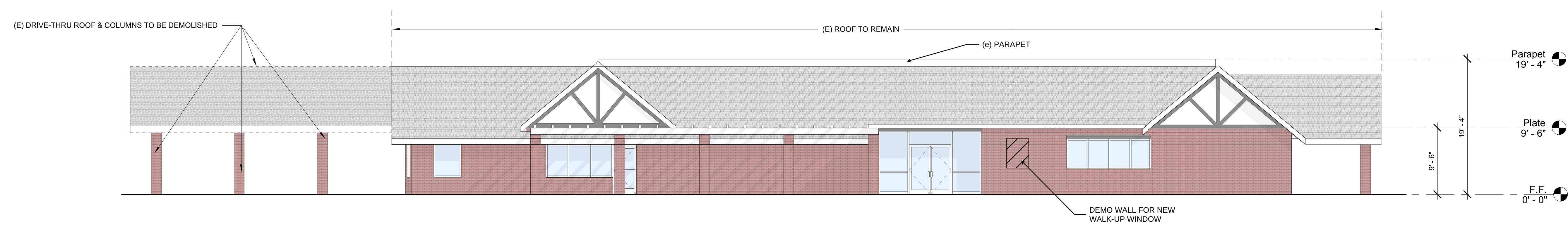
EXISTING EAST ELEVATION
