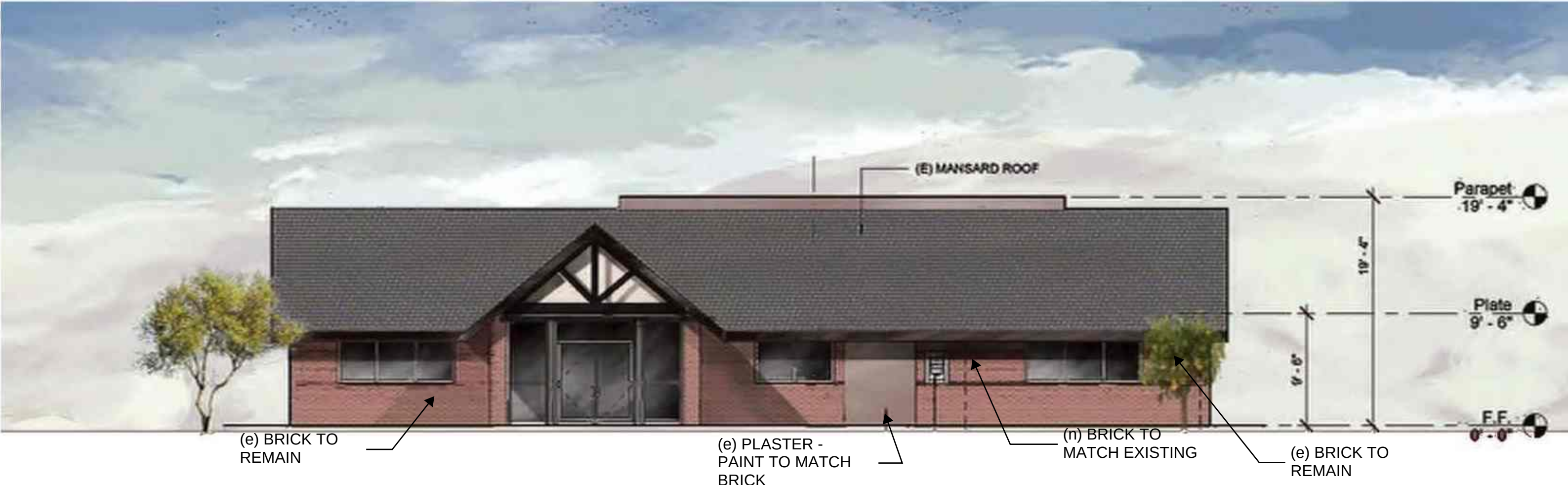
PRIOR APPROVED NORTH ELEVATION 1/8" = 1'-0"
